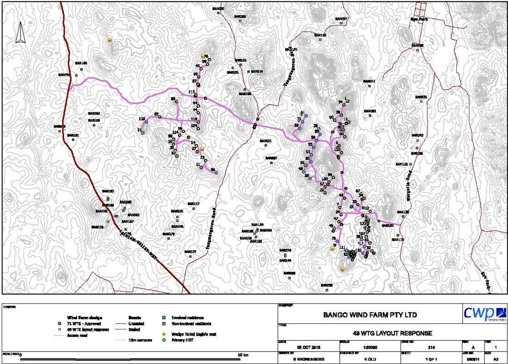
Figure 1: 71 versus 49 WTG layout
