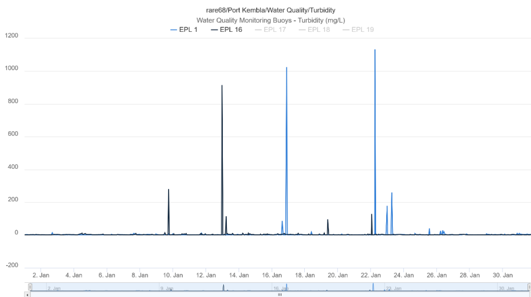
The above chart shows turbidity (NTU) observations at impact buoys EPL 1 and EPL16 for the reporting period.
