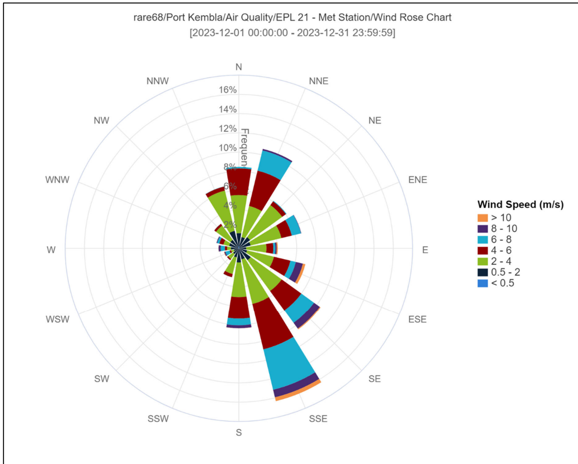
Figure 4-1 Wind Rose chart for the reporting period.
