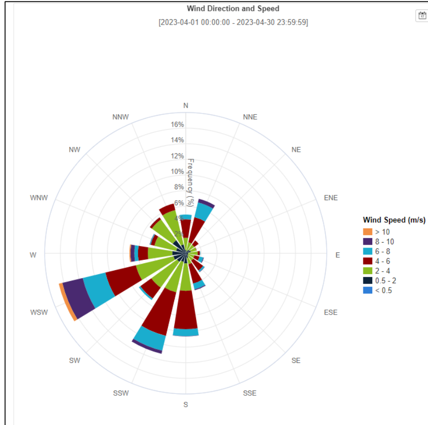
Figure 4-1 Wind Rose chart for the reporting period.
