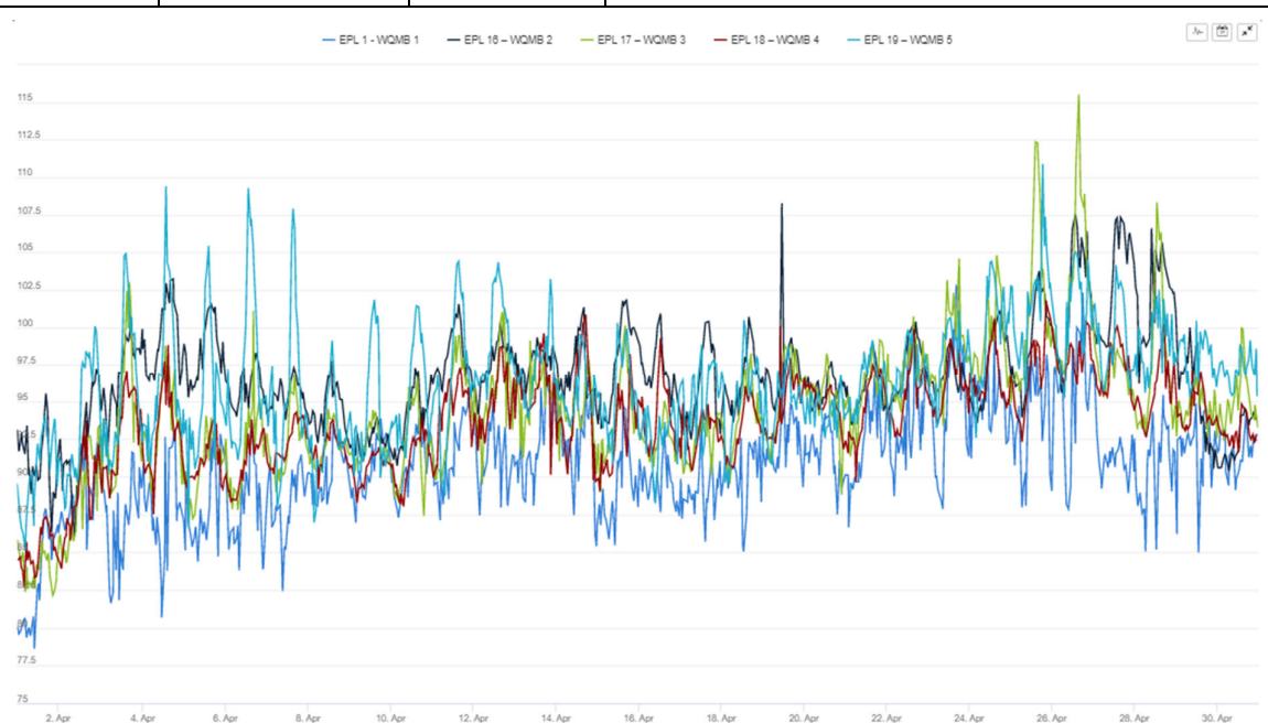
The above chart shows dissolved oxygen observations at impact buoys EPL 1, EPL 16 and EPL 17, as well as at background buoys; EPL 18 and EPL 19 for the reporting period.
