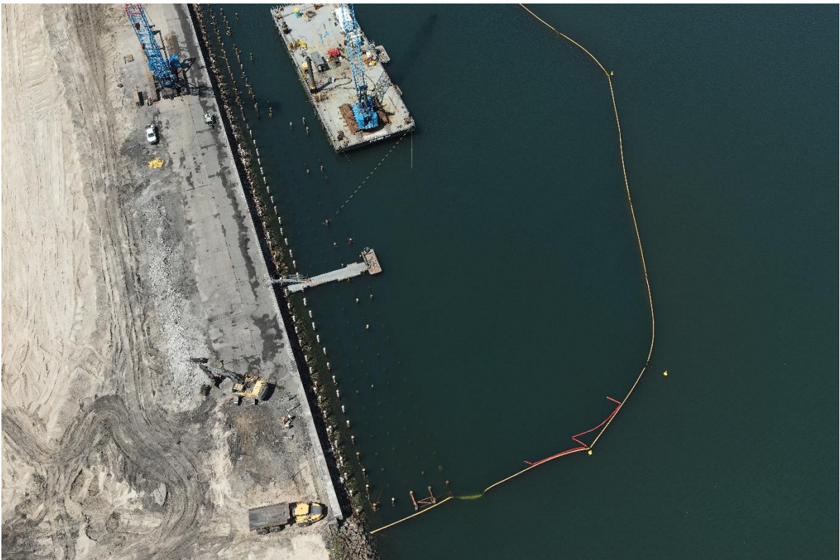
Photograph 2: View of remaining wharf piles at Berth 101.
